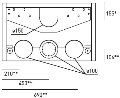
Rear view
